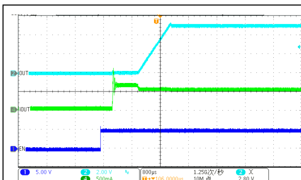
EN=L→H @ Vin=12V, Vout=5V, IOUT=300mA
