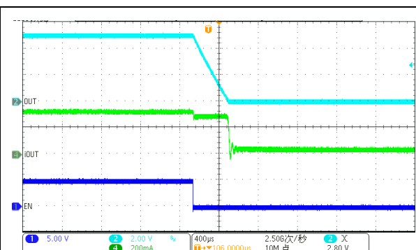
EN=H→L @ Vin=12V, Vout=5V, IOUT=300mA
