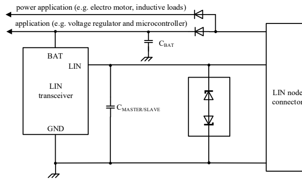
Typical application: ESD protection of one automotive LIN-bus line
